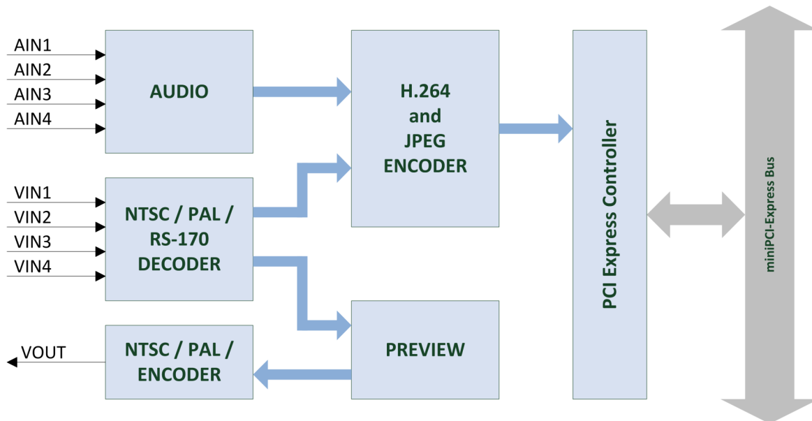
nanoH264-D4 Functional Diagram
